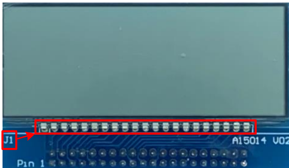
Top side of HY10000-AM01
